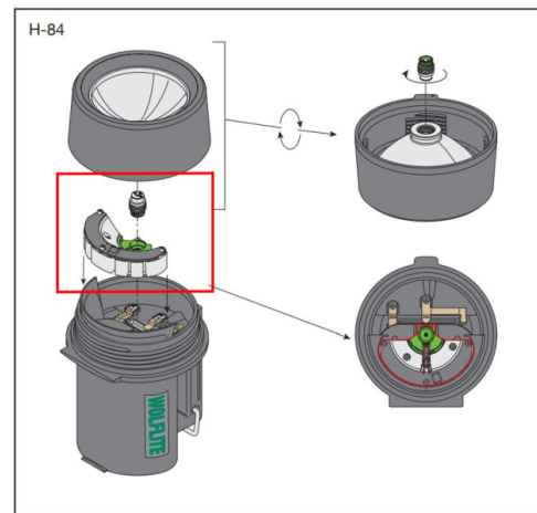
The H-84P LED Module; designed to upgrade existing H-4DCA bulb lamps to achieve the same outstanding performance as the brand new H-4DCALED handlamp
